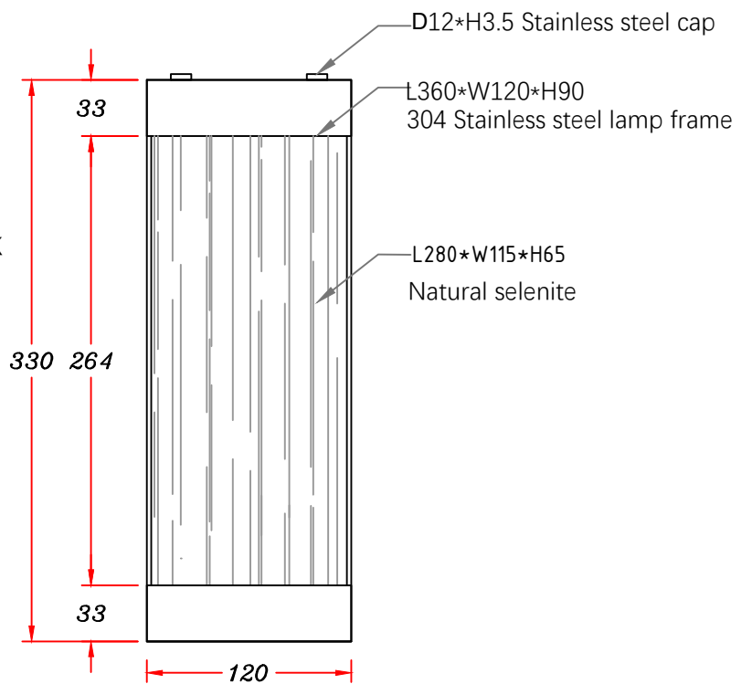
Side view
