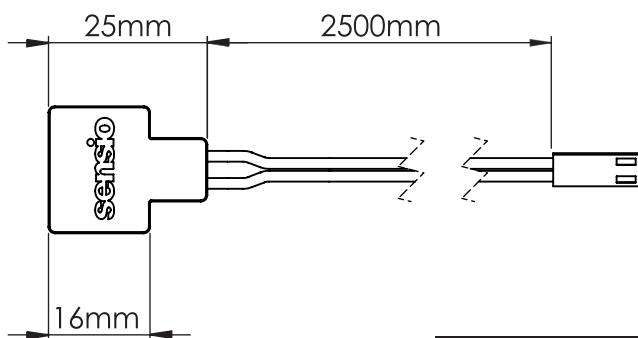
SE00037 Affinity - Driver Connection Lead
