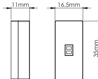
SE00047 Affinity - Magnetic IR Sensor
